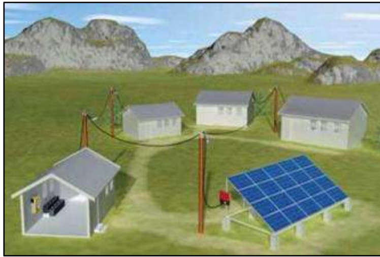
Figure 1- 2: Illustration of the components of solar mini-grids 2
