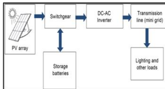
Figure 1- 1: Components of a solar mini-grid 1
