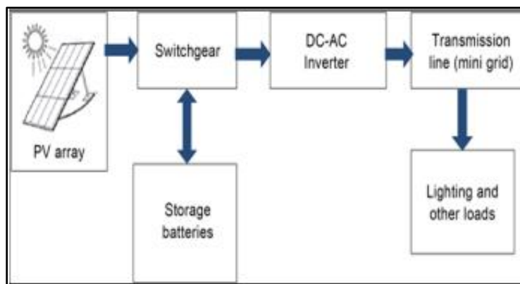
Figure 1- 1: Components of a solar mini-grid 1
