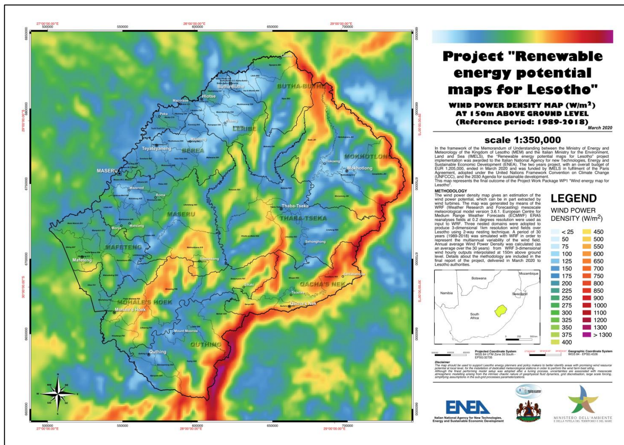
Figure A3: Wind Power Density (kW/m 2 ) for Lesotho at 150 m above ground level.
